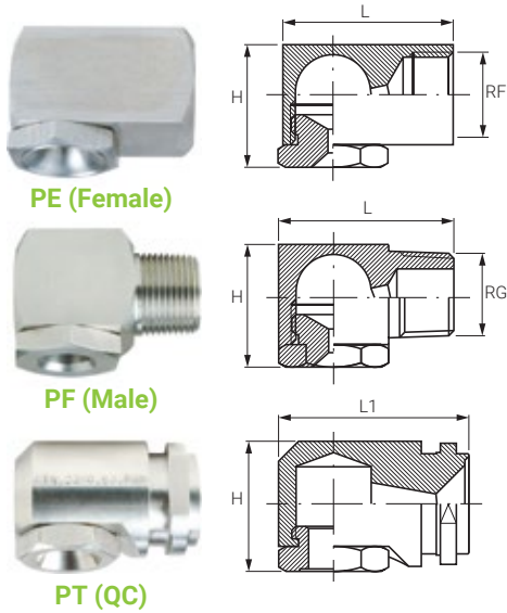
Spray section
