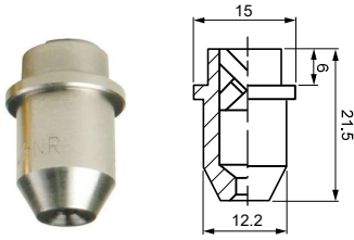
Above is outer shape of BX 1149 - BX 1372
