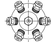
Cluster nozzle 7 nozzles type
