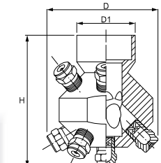
Cluster nozzle 7 nozzles type
