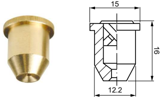
Above is outer shape of BX 1508 - BX 1743
