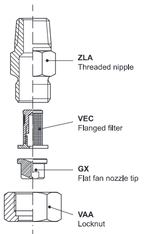
Assembly fittings
