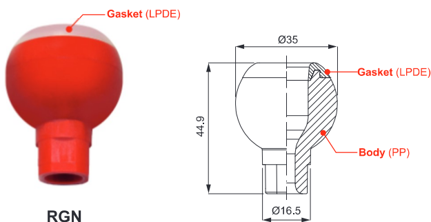
RGN Hollow cone nozzle
